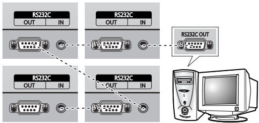
Example for Multiple Display Control connections
